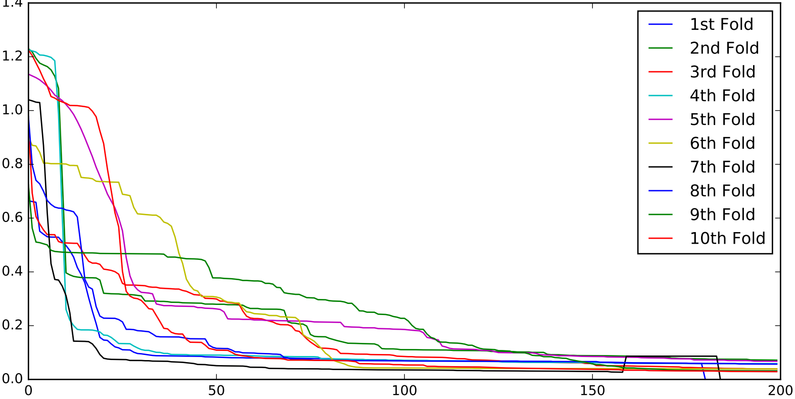
Training error of the best number of hidden units as function of BP iterations for each Fold
