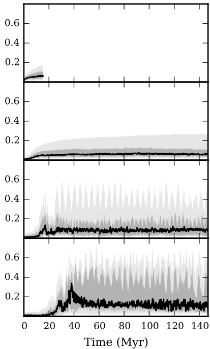
Eccentricity
