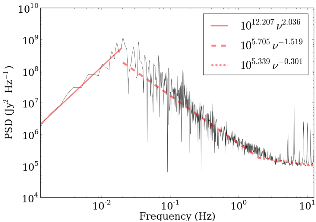
Figure 3.5 Fit to the power spectrum of a \sim 30 minute observation. Three independent power laws are fit to the data, with a fixed break at 0.02 Hz (below which the AC sampler removes signal) and a fitted break at higher frequency, near 2 Hz, where the power spectrum flattens towards white noise. The beam FWHM is at about 4 Hz using the standard scan rate of 120'' \text{ s}^{-1} .
