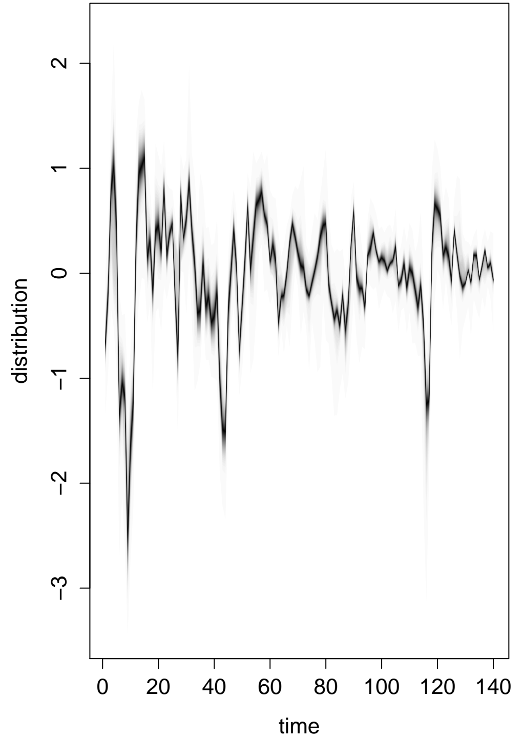
regression
