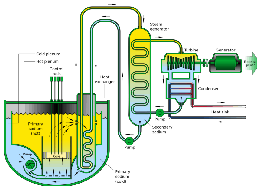
Figure 10: Fast Neutron Reactor
