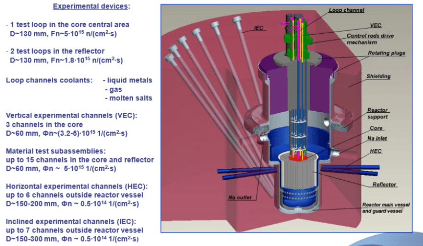
Figure 9: MBIR design and experimental capabilities
