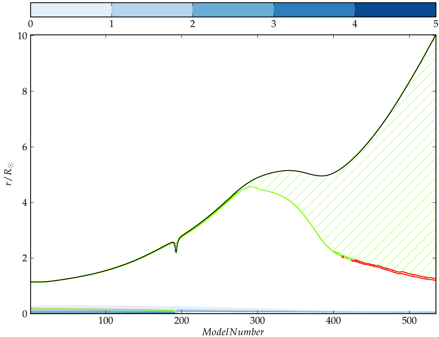
Nuclear Energy generation, Log (erg/g/s)
