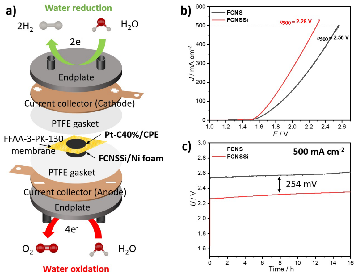
Figure 8 a) Zero-gap cell assembly using FCNSSi on Ni foam at anodic side against Pt/C (40%) on CPE at cathodic side, and b) LSV measurements, and c) chronopotentiometry test at 500 mA cm -2 for 16 h of both pristine FCNS and FCNSSi on Ni foam electrodes.
