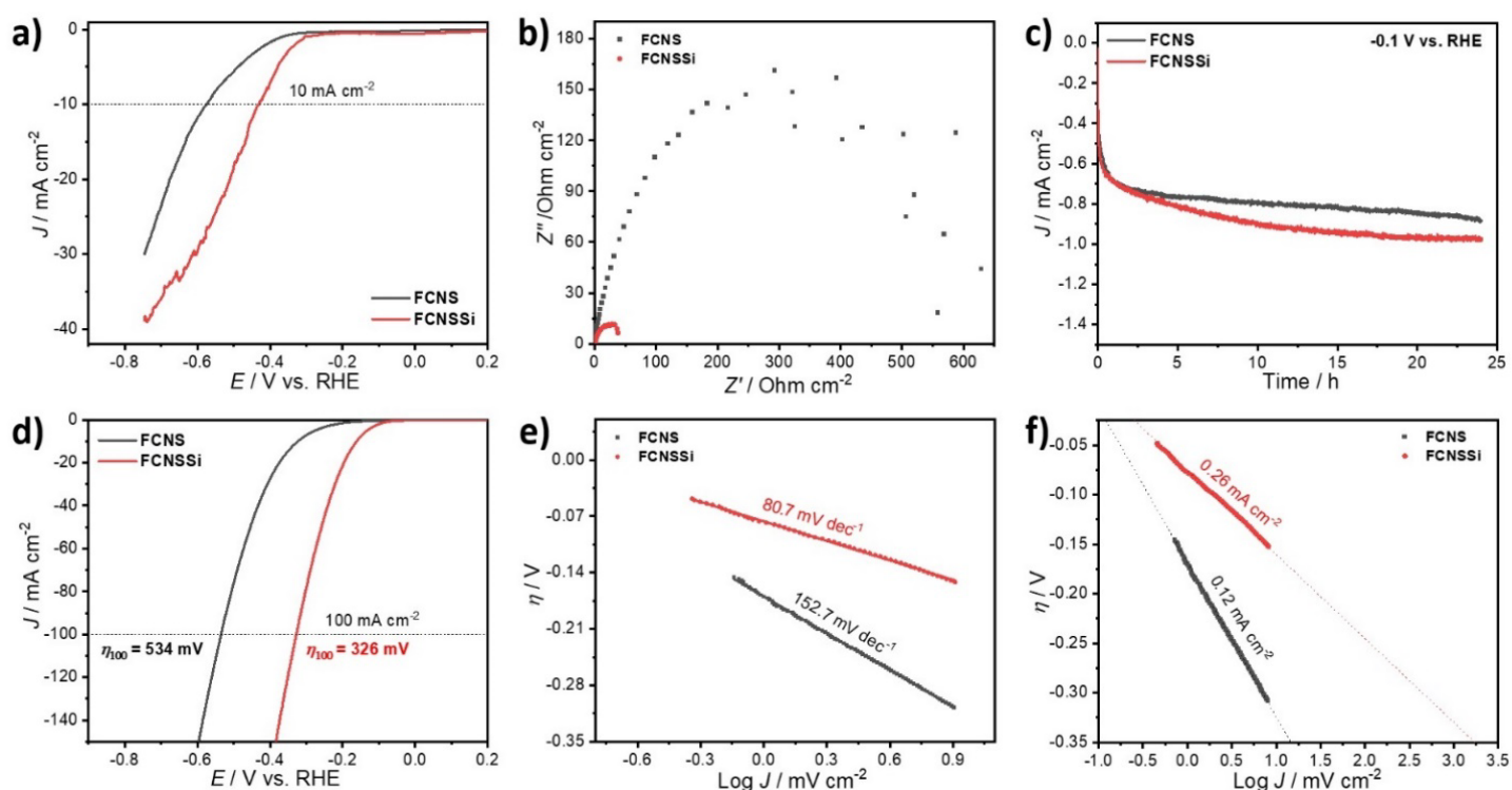
Figure 6 a) LSV curves of the as-prepared FCNS and FCNSSi in 0.5 M H 2 SO 4 solution at scan rate of 50 mV s -1 , b) EIS at -0.155 vs. RHE, c) chronoamperometry test at -0.1 vs. RHE, d) LSV curves after HER performance for 24 e, f) the derived Tafel plots of FCNS and FCNSSi samples on glassy carbon electrode.
