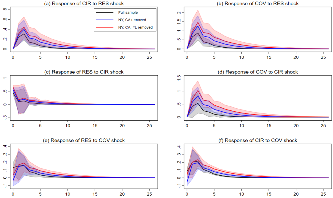
(b) Outliers
