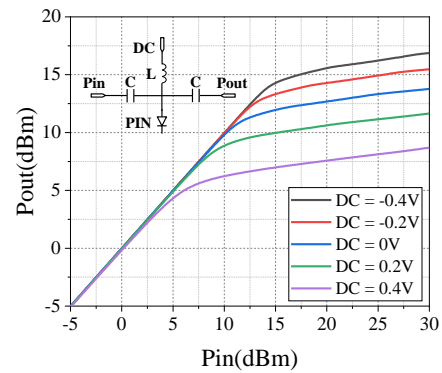
Fig. 2. Power input and output curves at different DC bias voltages
