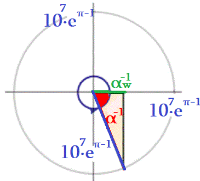
Figure 5. The angle in a^{-1} radians. The rotation vector moves in a circle of radius 10^7 \cdot e^{\pi-1} .
