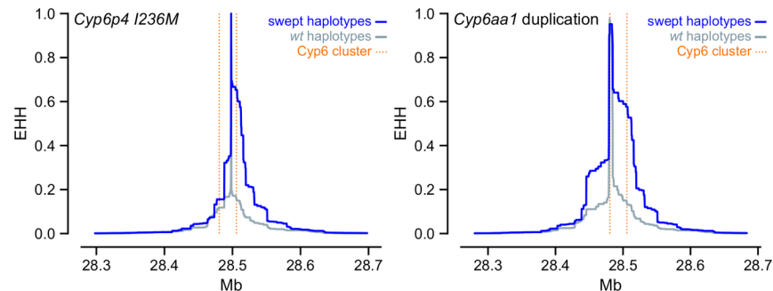
Figure 2. Selective sweep around the Cyp6aa/Cyp6p cluster in Anopheles gambiae from Uganda.
