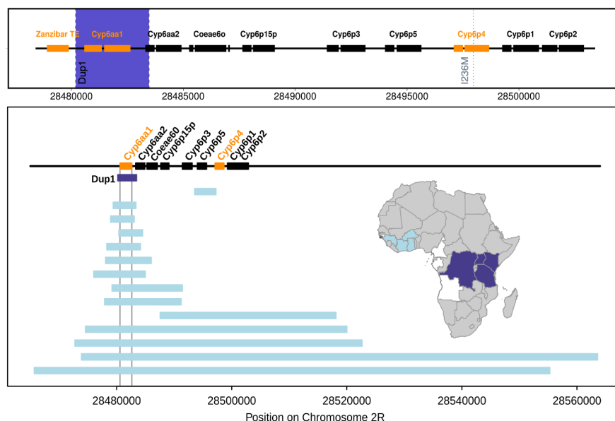
Figure 1. Schematic of the mutational events around the Cyp6aa/Cyp6p cluster on chromosome 2R in Anopheles gambiae . Upper panel shows the three mutational events observed in East and Central African samples. Orange indicates the genes/ transposable elements involved and the blue band the extent of the Cyp6aa-Dup1 CNV. The lower panel, redrawn from [20], shows the genomic extent and geographic distribution of the CNVs that have been observed around the Cyp6aa/Cyp6p cluster, 13 out of 15 include Cyp6aa1 . The dark blue shading on the map indicates the geographic extent of Cyp6aa-Dup1 . Data from Uganda, Kenya and DRC are reported extensively in the main text, in addition 27.4% (n=84) of Anopheles gambiae females sampled from northern Tanzania in 2018 were triple mutant carriers.
