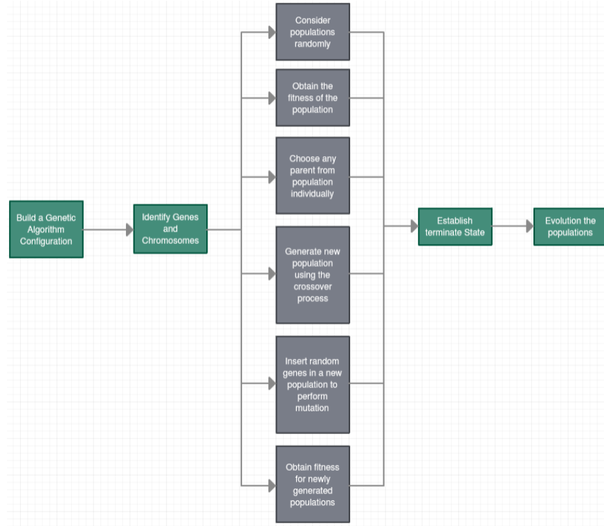
Fig. 4. Genetic Algorithm
