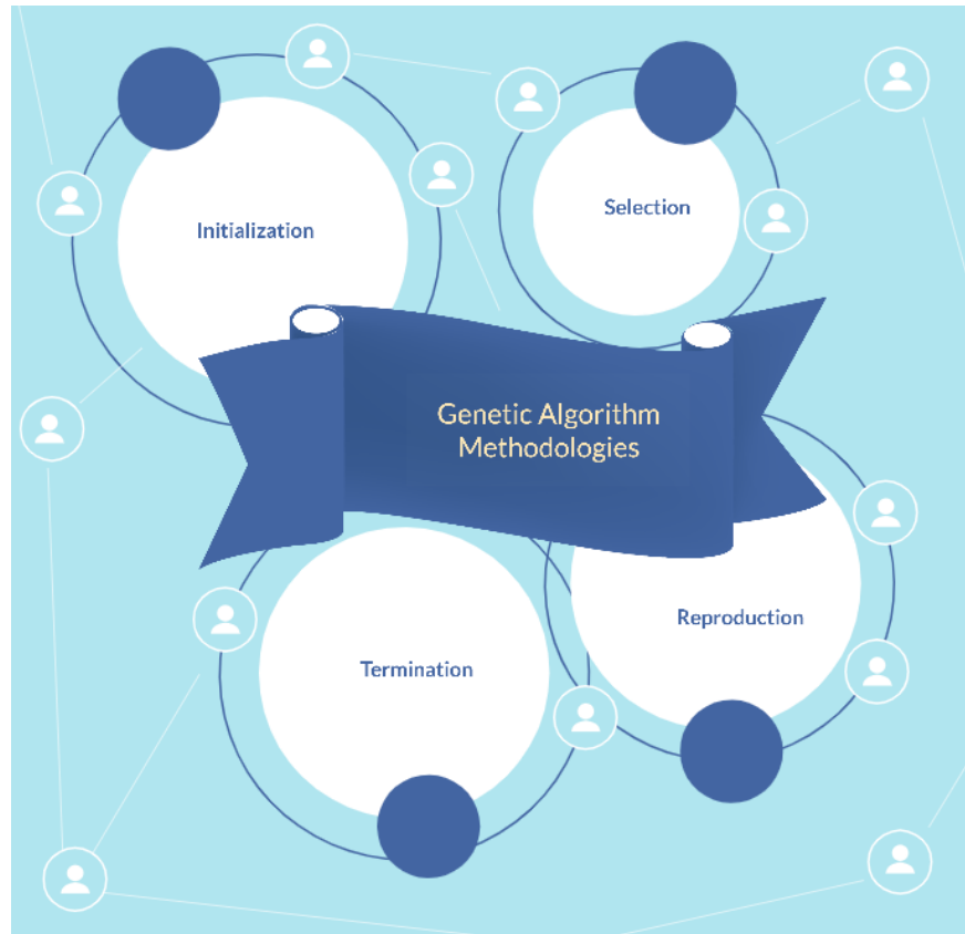
Fig. 5. Methodologies
