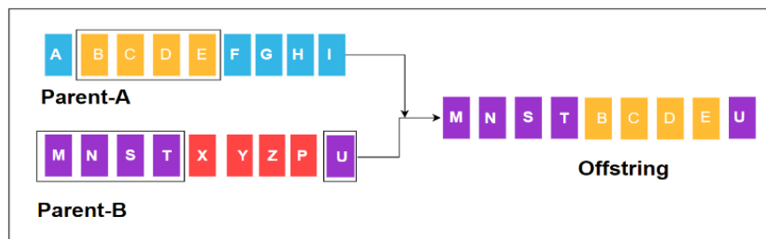
Fig. 2. Crossover operator
