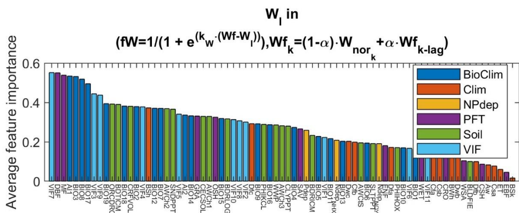
Figure S 9. The features sorted by the average normalized SHAP, LRP and PD for W_1
