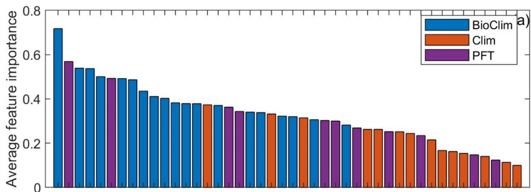
Figure S 10. The features sorted by the average normalized SHAP, LRP and PD for all parameters predicted using only bioclimatic variables, climate types and PFT.
