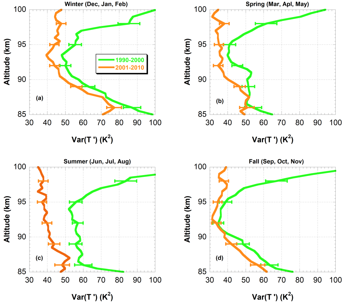
3. Profiles of the temperature fluctuations variances observed during a) winter (Dec, Jan, Feb), b) spring (Mar, Apr, May), c) summer (Jun, Jul, Aug), and d) fall (Sep, Oct, Nov) observed at CSU prior to current SWNA megadrought (1990-2000, green curves) and during the first ten years of the drought (2001-2010, brown curves). The error bars represent the rms uncertainties in
