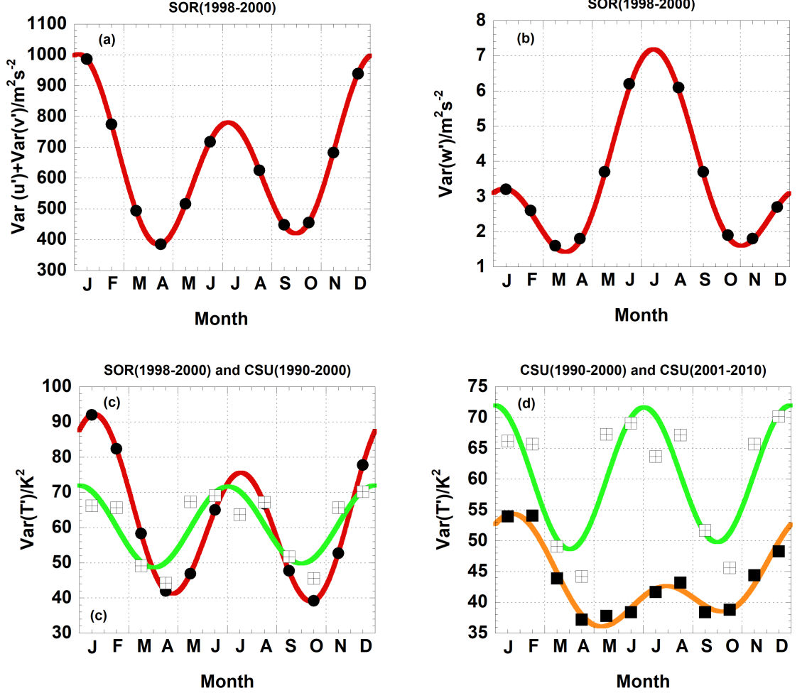
1. Seasonal variations of the mean fluctuation variances between 85 and 100 km. a) Horizontal wind variance at SOR (1998-2000), b) vertical wind variance at SOR (1998-2000), and c) temperature variance at SOR (1998-2000, red curve) and at CSU (1990-2000, green curve), all observed prior to the onset of the current SWNA megadrought. d) Temperature variance at CSU before (1990-2000, green curve) and during (2001-2010, brown curve) the megadrought. The symbols are the monthly means and the smooth curves are the mean plus AO and SAO harmonic fits to the data (Table 1).
