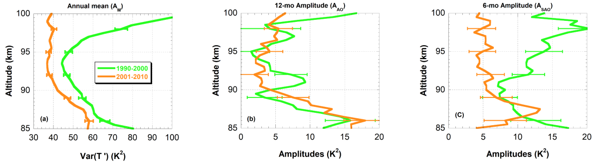
2. Profiles of the a) annual mean ( A_M ), b) 12-month amplitude ( A_{AO} ), and c) 6-month amplitude ( A_{SAO} ) of the harmonic fits to the temperature fluctuation variance observed at CSU prior to the current SWNA megadrought (1990-2000, green curves) and during the first ten years of the megadrought (2001-2010, brown curves). The error bars represent the rms uncertainties in the derived harmonic fit parameters.
