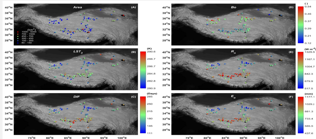
Fig. 2. The spatial distributions of lake area (A); lake surface temperature at the warmest three months (B); duration of ice-free season (C); Bowen ratio (D); net radiation (E); and evaporation during the ice-free season (F) of the 75 studied lakes.
