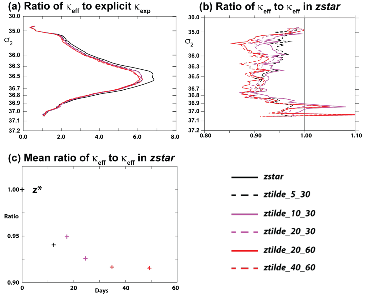
Figure 5. Ratios of global mean effective diffusivities \kappa_{\text{eff}} , evaluated in potential density classes: (a) ratios to the respective explicit diffusivity \kappa_{\text{exp}} ; and (b) ratios to \kappa_{\text{eff}} in zstar ; (c) Scatter plot of the mean \kappa_{\text{eff}} to \kappa_{\text{eff}} in z^* control in the density range 36.50 < \sigma_2 < 36.9 \text{ kgm}^{-3} against the harmonic mean of the two z -time scales (defining this to be zero for the zstar experiment).
