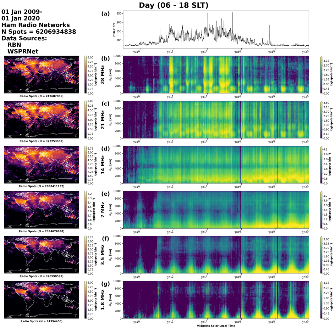
Figure 8: Daytime propagation for WSPRNet and RBN Observations for 2009 – 2020. The F10.7 Solar Flux Index is shown in panel (a). In this figure, only spots where the midpoint between the transmitter and receiver has a solar local time between 06 to 18 is shown.
