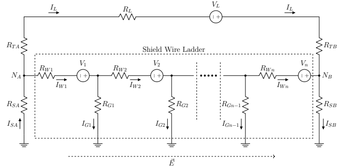
Fig. 1: Elementary circuit model to analyse the effect of shield wires on GICs through the transformers (from [2]).
