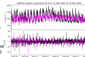
Fig 5 Helio1D output for the long-series data for benchmarking and calibration (purple) compared to observations (black).
