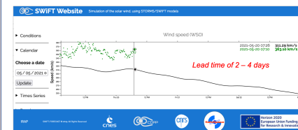
Fig 4 Example of the Helio1D pipeline output for the operational forecasting on the SWIFT website.
