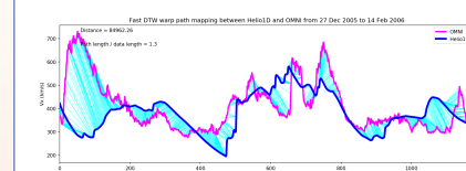
Fig 6 Example of the mapping between the predicted CIR structures and the OMNI using the FastDTW algorithm
