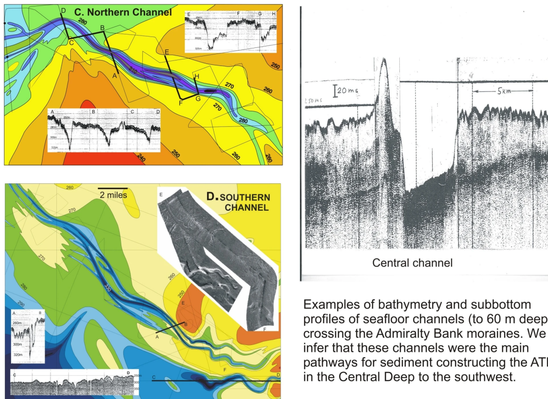
C and D. Examples of seafloor channels (to 60 m deep) crossing the Admiralty Bank moraines. We infer that these channels were the main pathways for sediment constructing the ATB in the Central Deep. See maps 1 and 2 for Areas C and D.
