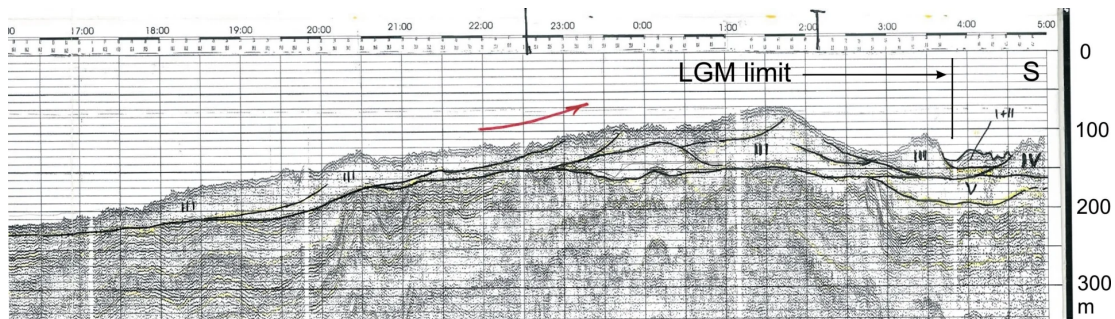
Seismic profile 7 east of the northern tip of Novaya Zemlya shows thrust moraines indicating southward movement from the SAT.
