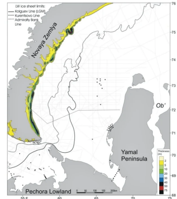
Fig.9. Isopach map of SSU-IIIc (Late Weichselian Admiralty Bank Till)
