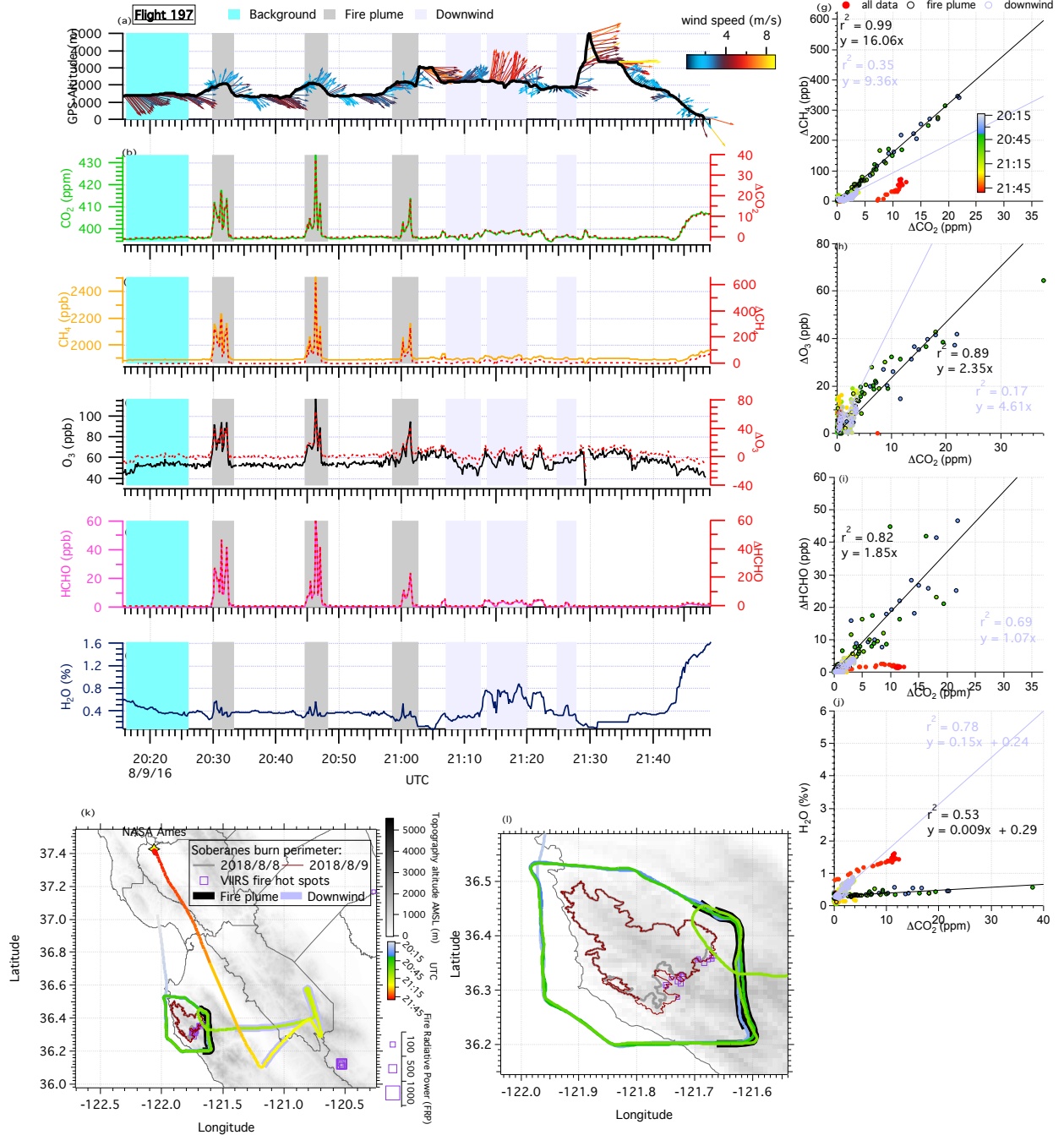
Figure 2. AJAX measurements during the Soberanes fire on August 9, 2016 (Flight 197). The aircraft altitude and wind speed/direction are shown in plot (a) followed by mixing ratios of trace gases in plots (b-f) (left y-axes) and enhanced mixing ratios (right y-axes). The gray bars represent the main fire plume, and the purple bars are aged plume interceptions. Cyan bars indicate the portion of the flight track assigned as background conditions. Scatter plots are shown for enhancements in (g) CH 4 , (h) O 3 , (i) HCHO, and (j) H 2 O vs CO 2 . The AJAX flight path colored by time and fire burn area for the flight day are shown on topographic maps (k-l), with VIIRS
