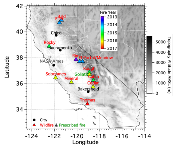
Figure 1. A topographic map with the location of fires measured by AJAX, colored by year.
