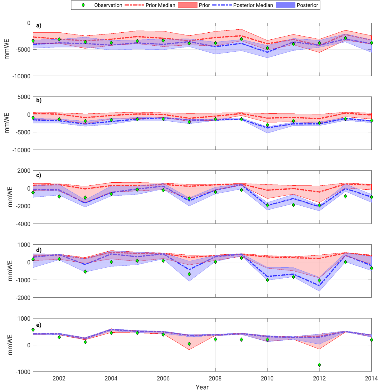
Figure 3: time series of the SMB for grid-cell co-located with the a) S5 and SHR, b) S6 and S7, c) S8, d) S9, and e) S10 stations along the K-transect. Values indicate year-over-year losses or gains in millimeter water equivalent (mmWE). The prior and posterior estimates are
