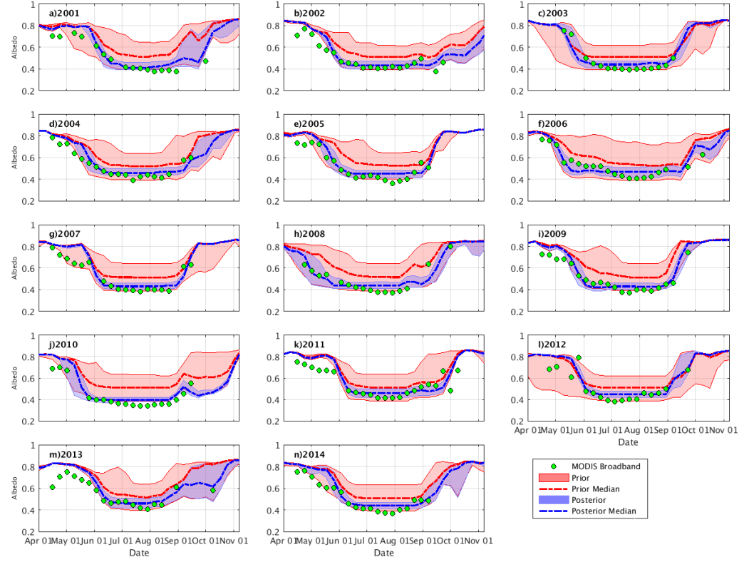
Figure 2: Time series of albedo (-) for the grid cell co-located with stations S5 and SHR for 2001 to 2014. The red and blue shaded areas represent the prior and the posterior uncertainty band (IQR) and the red and blue dash lines represent the median of the prior and posterior, respectively. The green circles represent the satellite-derived 16-day albedo.
