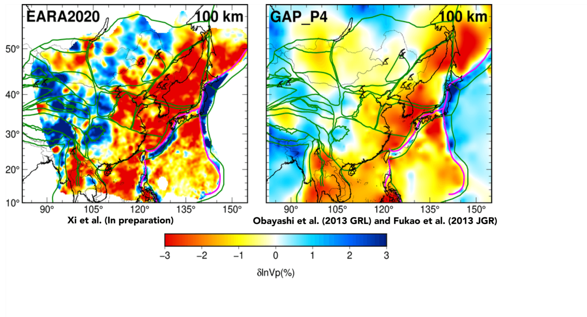
Fig. 6 Model comparison between EARA2020 and GAP_P4 at 100 km depth. The velocity contrast of EARA2020 is sharper and the slab interface stands out more. Intraplate tectonic structures like the Ordos block in northern China and the Sichuan Basin in south-west China have a clear high-V anomaly. Model EARA2020 has more small-scale structures with larger amplitude for the wave speed anomaly.
