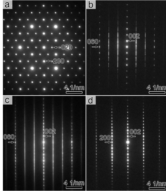
Figure 3. Amesite SAED patterns along (a) [001], (b,c) [100] and (d) [010]. The patterns were indexed with a pseudo-orthogonal unit cell. Strong streaks were observed at (0kl) with k=6n\pm2 , where k and n are integers. The presence of (00l) diffraction spots for odd l in (c) and (d) is caused by multiple diffraction, as verified by tilting the sample 6^\circ\sim10^\circ away from the zone axis along the (00l) Kikuchi lines. The SAED patterns of lizardite were similar, so not shown here.
