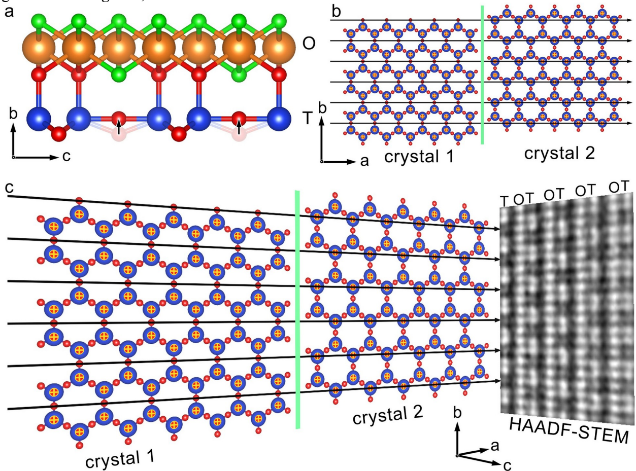
Figure 6. (a) Projection of one TO layer along [100] . Si, Mg, O and hydroxyls are represented by blue, yellow, red and green balls. For the oxygen columns to locate at the same level of Si would completely disrupt the tetrahedral sites. (b) Tetrahedral sheets viewed along [001] . Red balls with crosses are apical oxygen atoms of the tetrahedra. Red balls and those with crosses are below and above the projection plane (Si balls), respectively. The same tetrahedral sheet in crystal 2 is shifted by 1/3b ( -1/3b also works) relative to that in crystal 1. Green line illustrates the interface. To guide the eye, projection of Si atoms along [100] onto the HAADF-STEM image is illustrated by the long black arrows.
