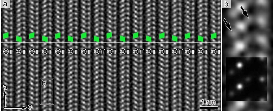
Figure 4. HAADF-STEM images viewed along [010] . In (a), the tilts of octahedral sheets in each TO layer are sketched with green parallelograms. The tetrahedral cations in adjacent TO layers are located at the same horizontal line, indicating no interlayer shifts along the a -axis. The framed region is enlarged and shown in (b), where the simulated image is superimposed. Black arrows mark the oxygen columns. The basic features in the images of amesite and lizardite are the same, so only the images of amesite are presented here.
