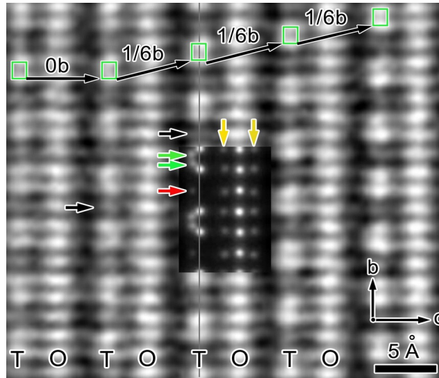
Figure 5. (a) HAADF-STEM image viewed along [100] . Cation pairs in the tetrahedral sheets are highlighted by green boxes and relative interlayer shifts between two TO layers are illustrated by long black arrows. The inset at the center is a simulation image. Green, red and yellow arrows mark the contrast due to different oxygen atomic columns in the simulation image. However, the contrast due to these oxygen atoms cannot be resolved in the experimental image. Interestingly, for the columns between tetrahedral cation pairs, there is contrast variation in the experimental image, as indicated by the short black arrows. The greater contrast indicated by the arrow on the left is because shifts of \pm 1/3b bring more tetrahedral atoms there, as shown in Fig. 6 . The basic features in the images of amesite and lizardite are the same, so only the images of amesite are presented here.
