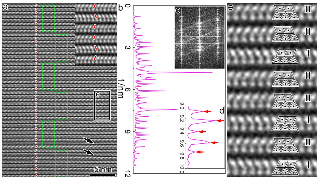
Figure 11. (a) HAADF-STEM image of 8-layer lizardite. A zoom-in image is shown in the inset. Red lines denote the tilt of octahedra. Green boxes indicate the 8-layer repeat of the tilt pattern. (b) Intensity profile along the arrow in the fast Fourier transformation in (c). (d) is enlarged from (b). Red arrows mark five peaks. (e) is a higher magnification view of a region in (a), showing one stacking unit with the (II,II,I,II,II,I,II,I) tilt pattern. The triangles and parallelograms with dots at the centroid illustrate the tetrahedra and octahedra, respectively.
