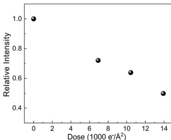
Figure 2. Intensity evolution with accumulated electron dose. The intensity is normalized to the value in the SAED pattern recorded before the irradiation experiment. The data shown were for an amesite sample, but the results apply for lizardite as well.
