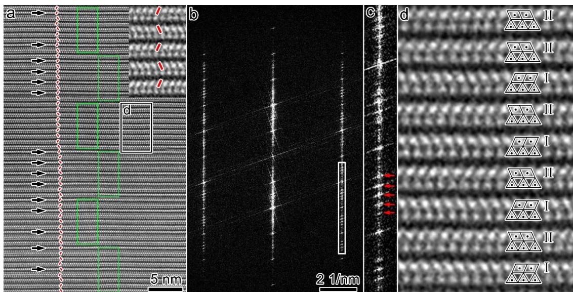
Figure 12. (a) HAADF-STEM image of 9-layer lizardite. Many lizardite layers have transformed to chlorite layers. A zoom-in image is shown in the inset. Red lines denote the tilt of octahedra. Green boxes indicate the 9-layer repeat of the tilt pattern. (b) Fast Fourier transformation of (a). (c) is enlarged from the framed region in (b). Red arrows mark five spots used for periodicity calculation. (d) is zoomed from (a), showing one stacking unit with the (II,II,I,II,I,II,I) tilt pattern. The triangles and parallelograms with dots at the centroid illustrate the tetrahedra and octahedra, respectively.
