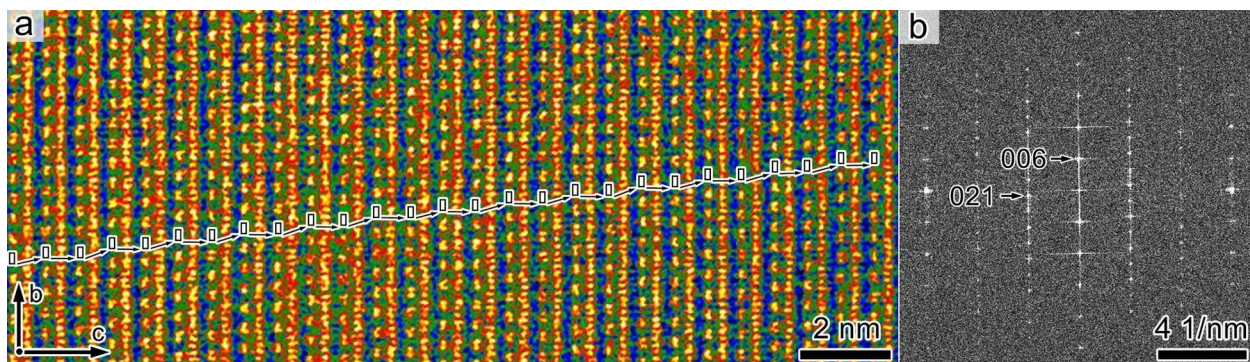
Figure 8. (a) HAADF-STEM images of 6R_2 amesite. The ordered 6R_2 stacking extends over tens of nanometers (only several unit cells are shown). Small boxes mark the tetrahedral cation pairs, and arrows denote the interlayer shifts. A false-color temperature map is used for clearer visualization. (b) Fast Fourier transform of the HAADF-STEM image in (a). Spots were indexed based on the 6R_2 structure.
