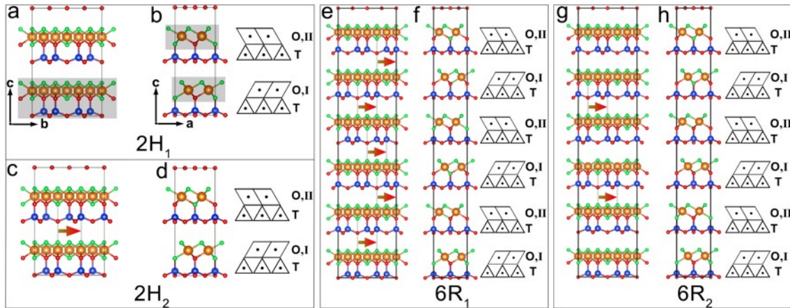
Figure 1. Illustration of four common polytypes of sheet serpentine. (a,b) 2H_1 , (c,d) 2H_2 , (e,f) 6R_1 , (g,h) 6R_2 . The projections in (a), (c), (e) and (g) are along [100] , while those in (b), (d), (f) and (h) are along [010] .
