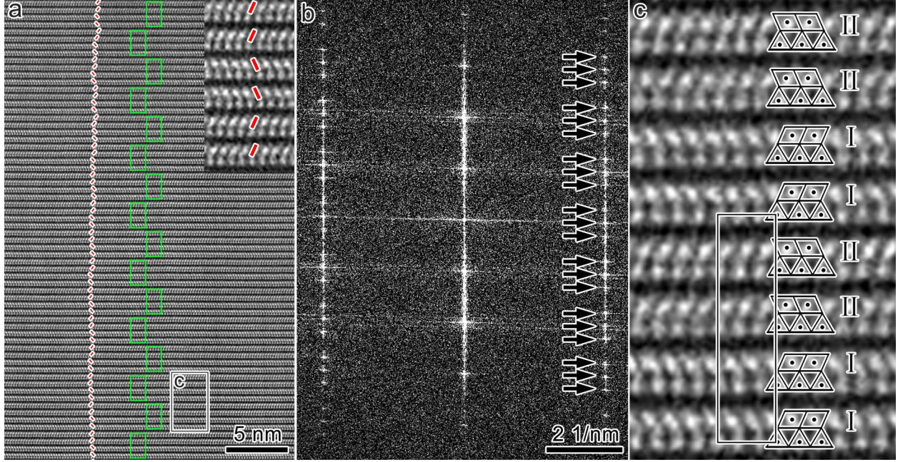
Figure 10. (a) HAADF–STEM image of 4-layer lizardite. A zoom-in image is shown in the inset. Red lines denote the tilt of octahedra. Green boxes indicate the 4-layer repeat of the tilt pattern. (b) Fast Fourier transformation of (a) in which arrows indicate spots representing 30.2 Å periodicity. (c) Higher magnification of a region from (a), showing two stacking units with the (II,II,I,I) tilt pattern. Triangles and parallelograms with dots at the centroid illustrate the tetrahedra and octahedra, respectively. A unit cell is highlighted with a black rectangle.
