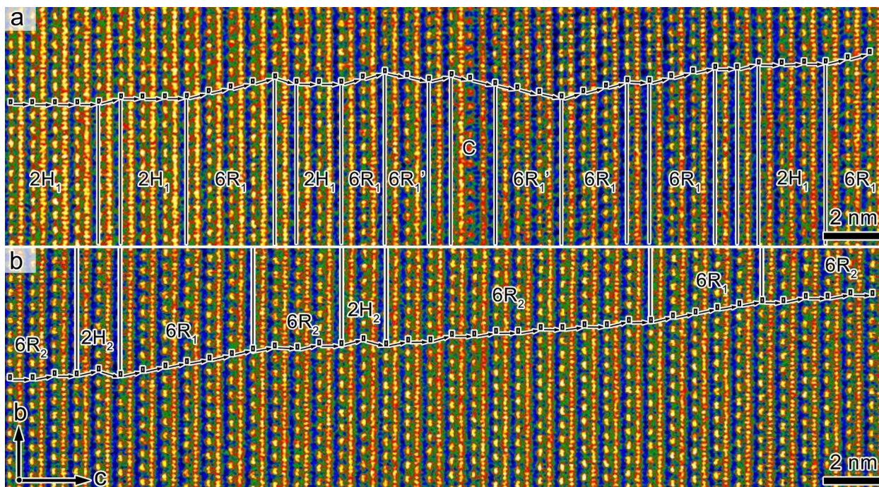
Figure 7. HAADF-STEM images showing co-existence of (a) 2H_1 and 6R_1 , (b) 6R_2 , 6R_1 and 2H_2 stacking in amesite. The region denoted as C in (a) is a chlorite layer. Small black boxes mark the tetrahedral cation pairs and arrows denote the interlayer shifts. A false-color temperature map is used for clearer visualization.
