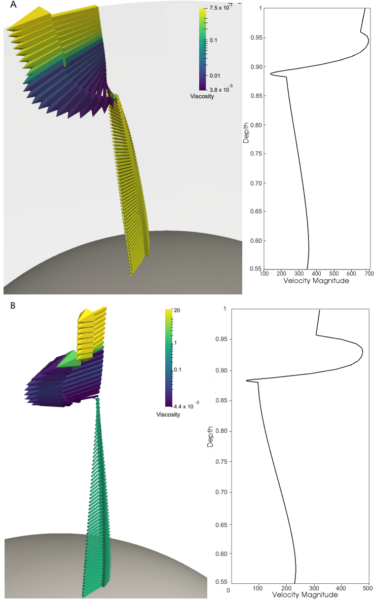
Figure 4. Local velocity profiles for for cases A) \sigma_y = 2.8 * 10^3 . and B) \sigma_y = 5 * 10^3 . Left: Perspective view on local profile results where colors indicate viscosity. Right: 2D velocity profile from the matching left image. indigo arrows show asthenosphere depths where asthenosphere flow in both cases rotates away from lithosphere flow and locally leads plate velocities.
