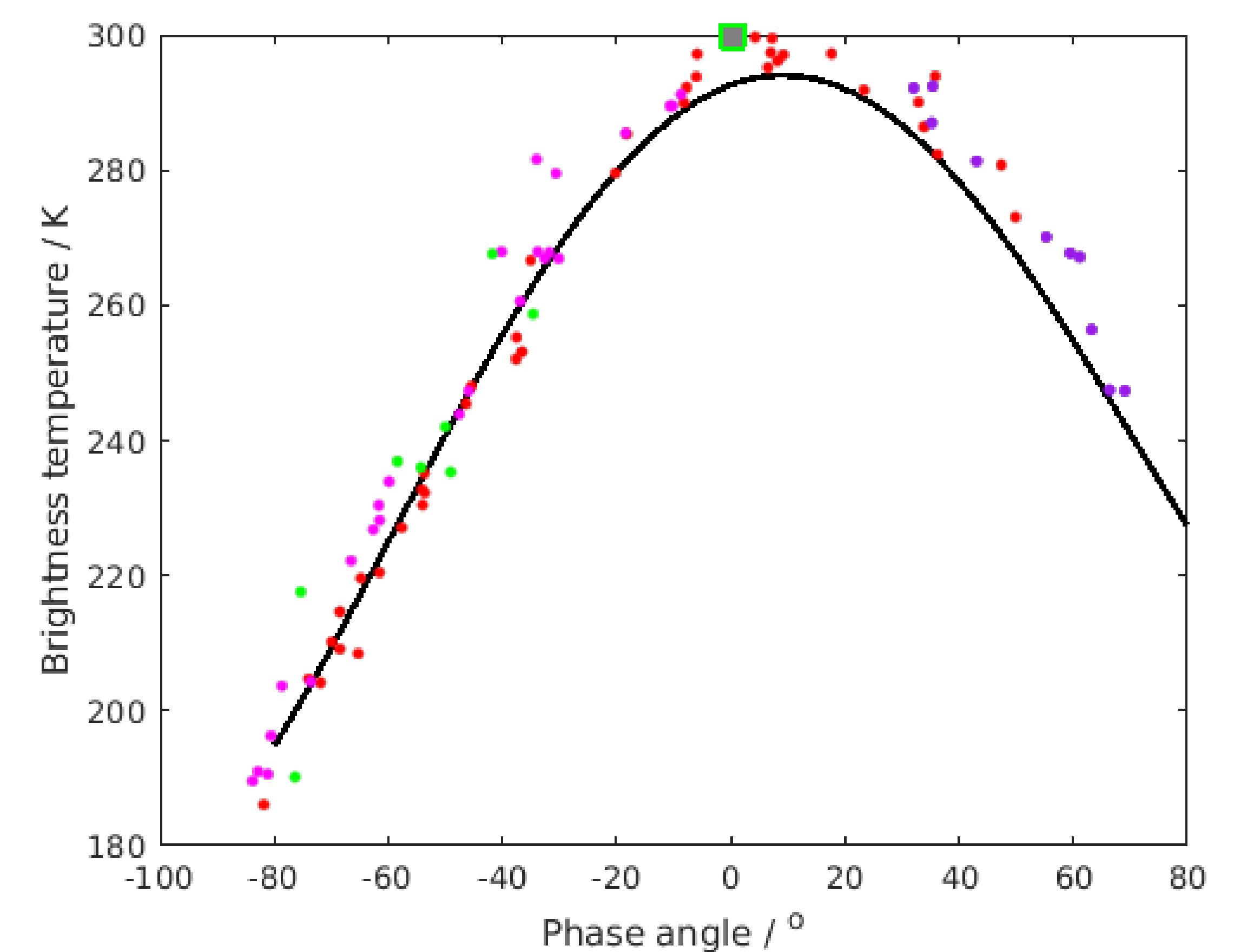
Disk-integrated T_b (89 GHz) of the Moon for different phase angles. Green: AMSU-B on NOAA-16, red: MHS on NOAA-18, magenta: MHS on NOAA-19, blue: MHS on MetOp-A, gray square: ATMS on NOAA-20, solid line: model by Keihm (1984).
