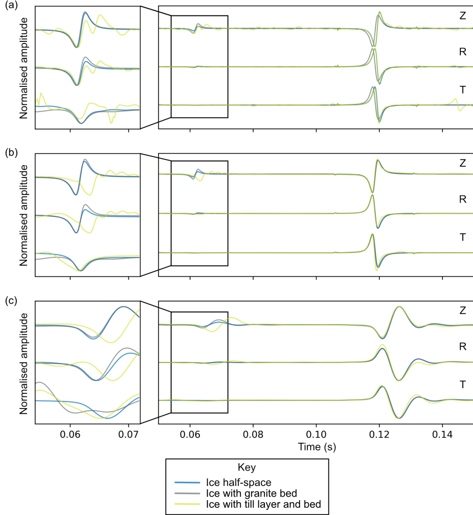
Figure 10. The effect of attenuation and bandpass signal filtering on the ability to resolve a till layer for the Rhonegletscher icequake. The seismograms are for a DC source with a strike, dip and rake of 85.1^\circ , 24.4^\circ and -90.0^\circ , respectively, arriving at station RA54. a) Synthetic seismogram for negligible attenuation. b) Seismograms for attenuation, but no filtering. The ice Q factors are 600 for P and 300 for S, and till Q factors are 25 for P and 1 for S. c) Same as (b) except a bandpass filter is applied between 5 and 100 Hz . The till layer is 2 m thick. The velocities of the media and source-time function used are as in the other inversions in this study.
