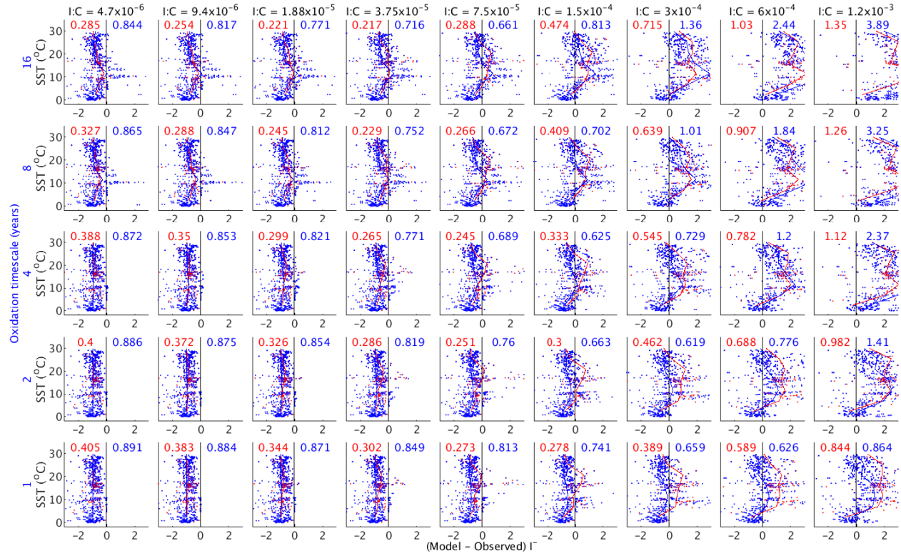
Figure 4: Normalised difference between modelled and observed iodide concentrations, as a function of SST, for a range of I:C production ratios, and iodide oxidation timescales. The RMS errors for coastal (< 200 m) and open ocean (> 200 m) locations are shown in red and blue respectively.
