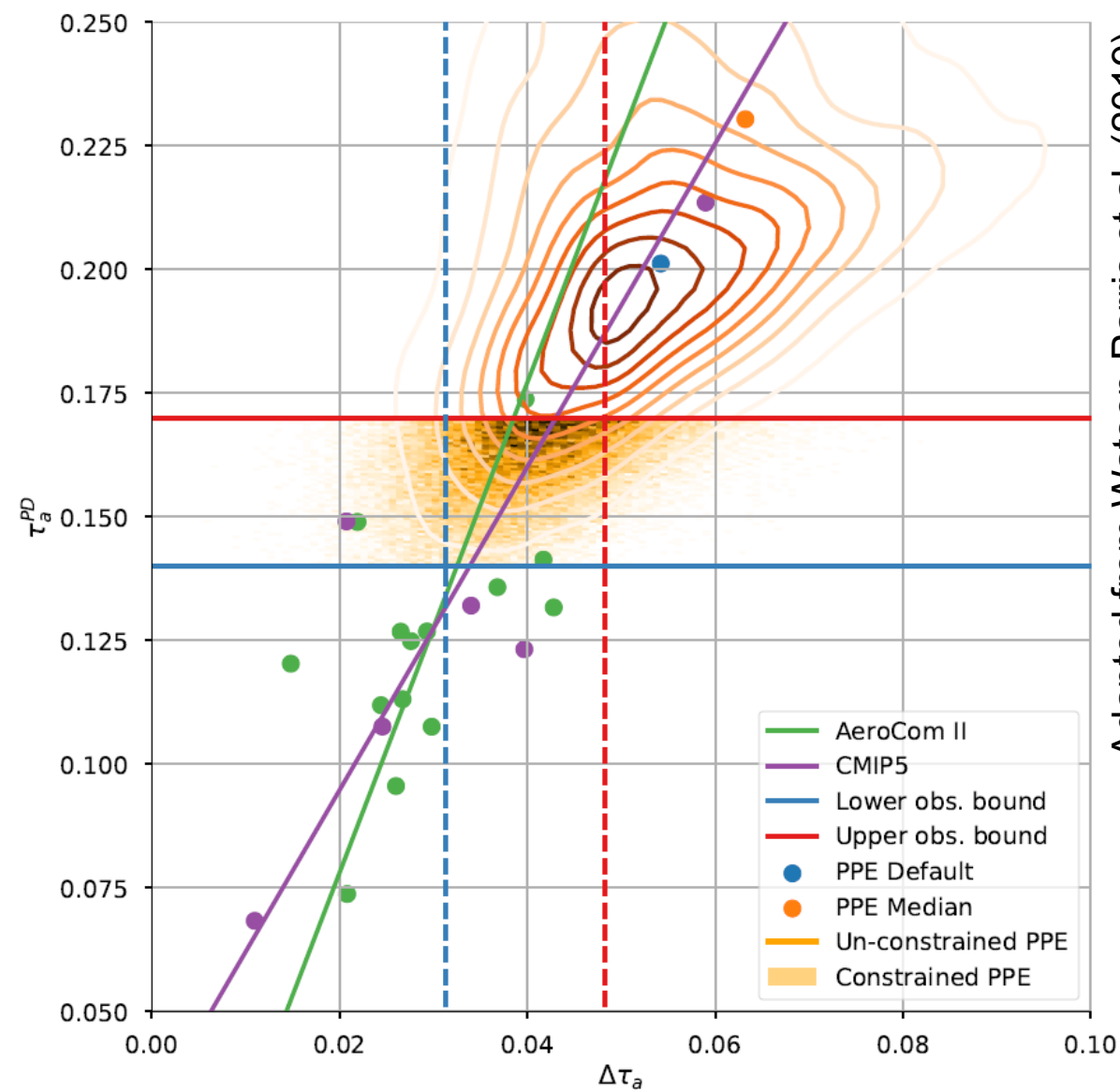
Figure 1: Distributions, standard deviation and best-fit lines of the present-day aerosol optical depth \tau_a^{PD} against the industrial-era change in aerosol optical depth at 0.55 \mu\text{m} , \Delta\tau_a between 1850 and present-day.
