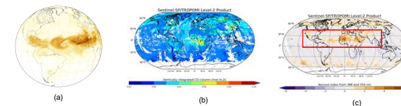
Figure 6: The transatlantic dust plumes (in the red box) on July 1 st , 2018. (a) is the GEOS-5 simulation. (b) and (c) are S5P/TROPOMI CO and UVAI L2 products.
